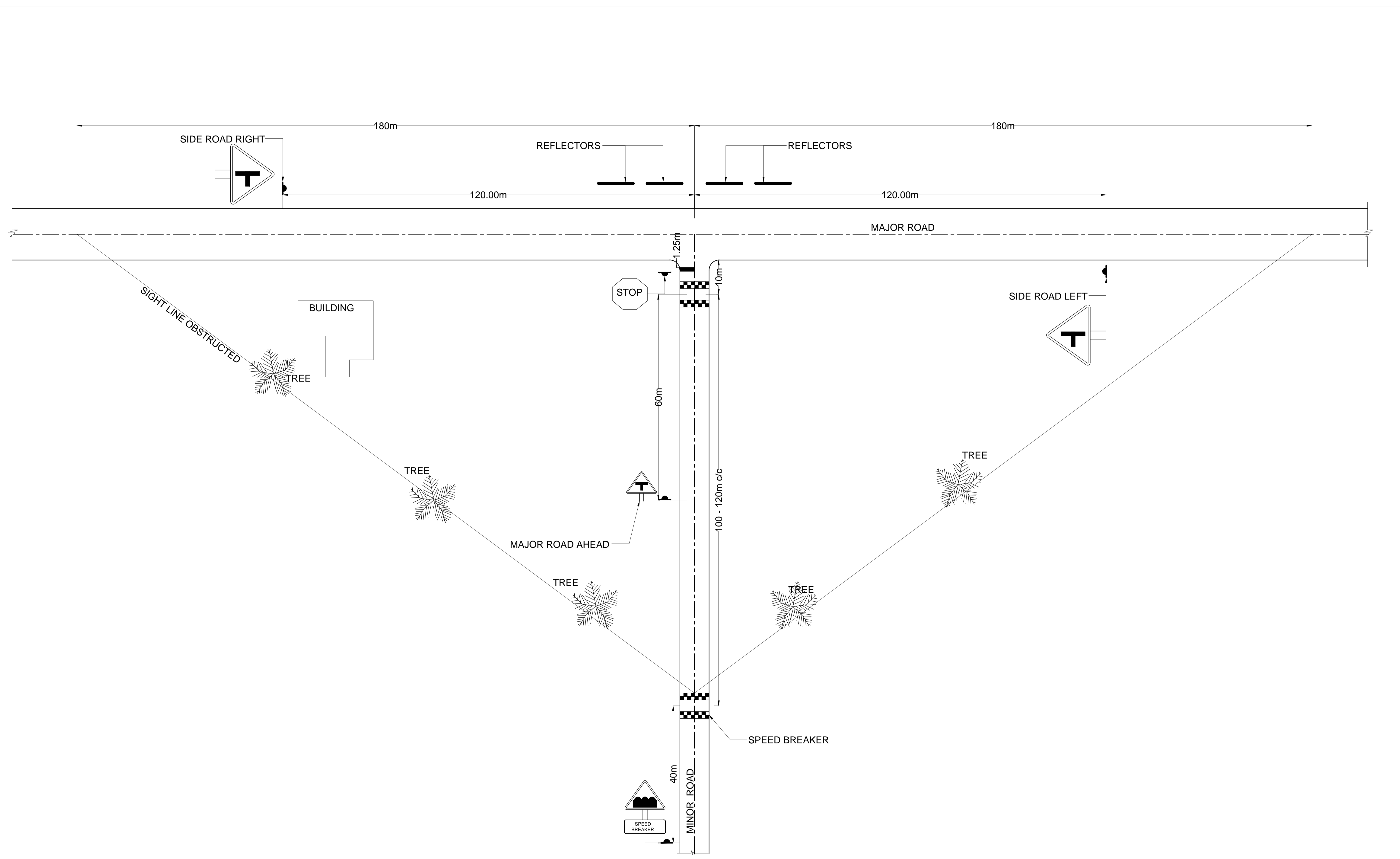
SPEED BREAKERS AT T- INTERSECTION
