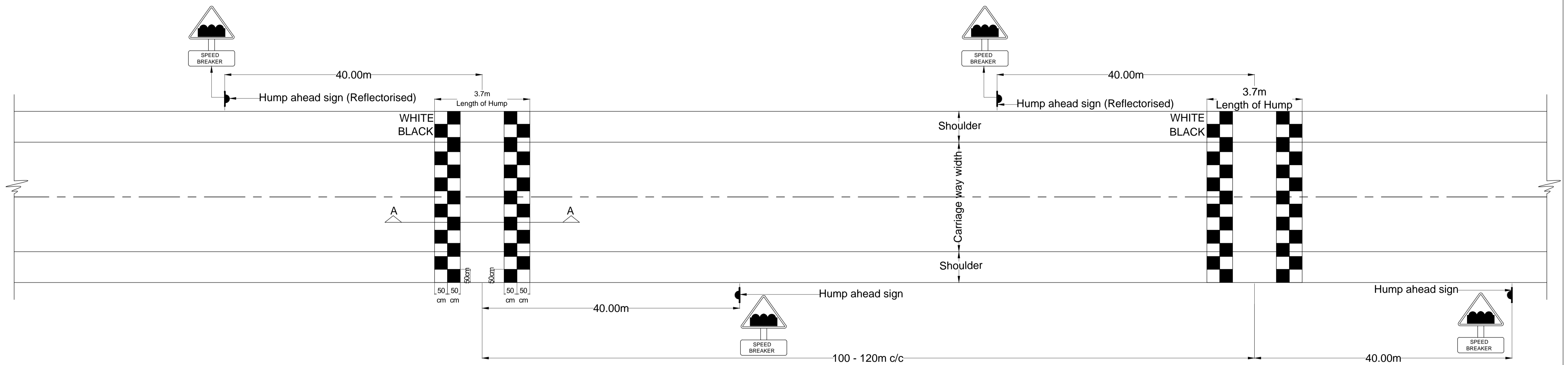
RECOMMENDED PLACEMENT OF HUMP/HUMPS IN MID-BLOCK SECTION. HUMP MARKING IN CHEQUERED PATTERN AND SIGN BOARD LOCATIONS
