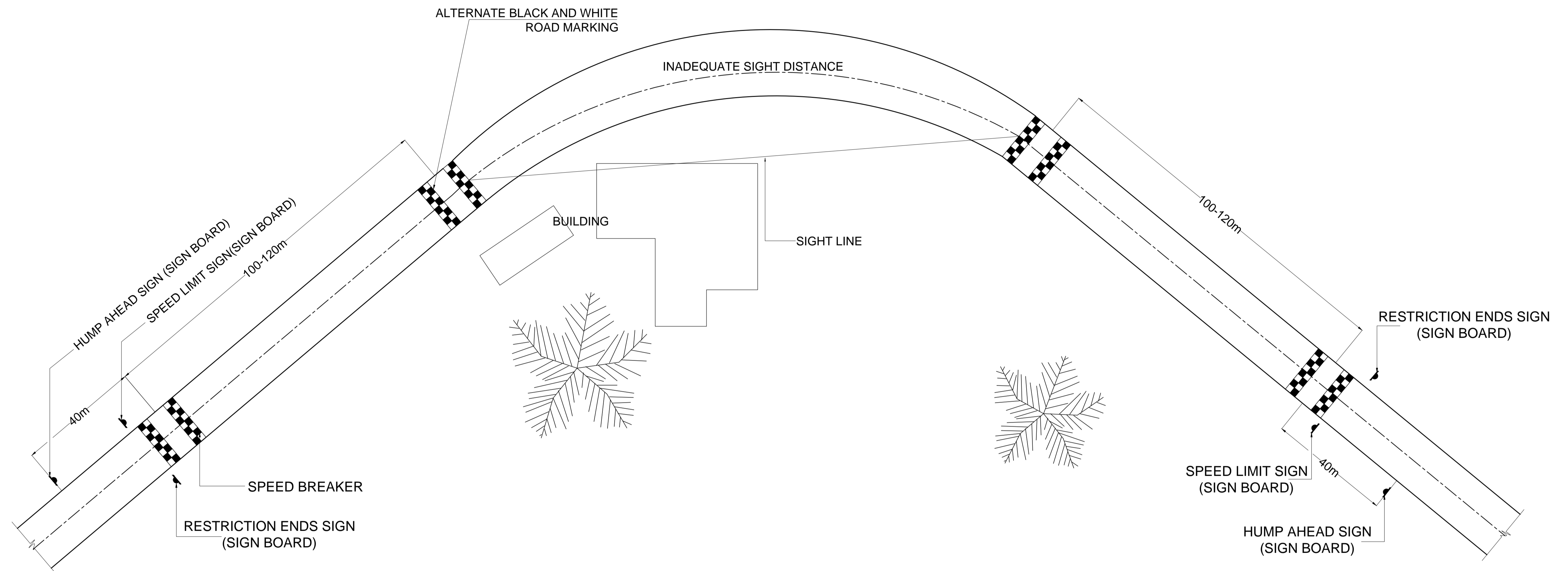
PLAN OF SPEED BREAKERS ON APPROACH TO A SHARP CURVE
