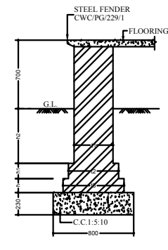
SECTION AT PLATFORM
