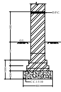
SECTION AT PARTITION WALL
