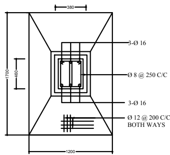
PLAN COLUMN -C 1
