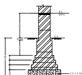
SECTION AT LONG WALL
