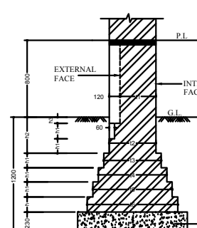
SECTION AT GABLE WALL
