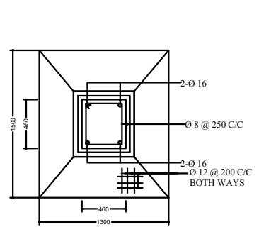
PLAN COLUMN -C 2
