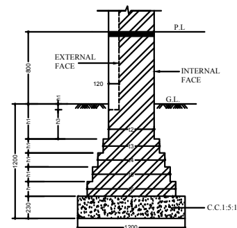
SECTION AT GABLE WALL FOR 250 THK. SIZE BRICK
